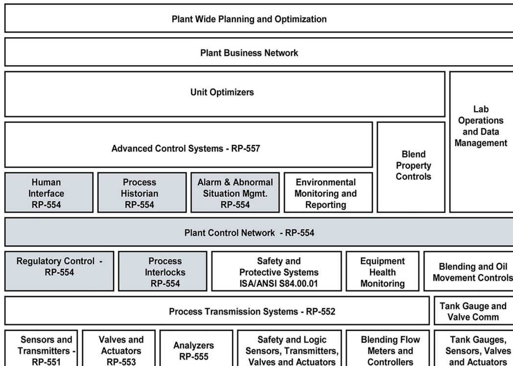
Figure 1—Oil and Gas and Refinery Process Control—Automation Functions
